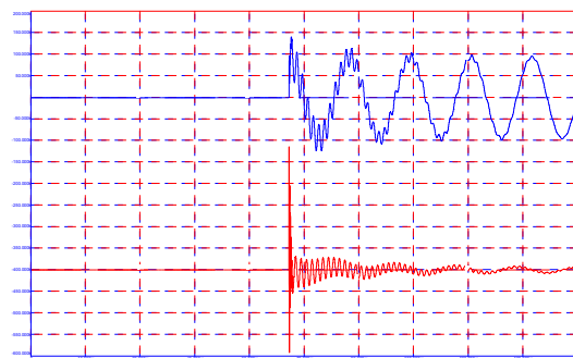
Voltage and Current for Energization of 2 nd Bank
