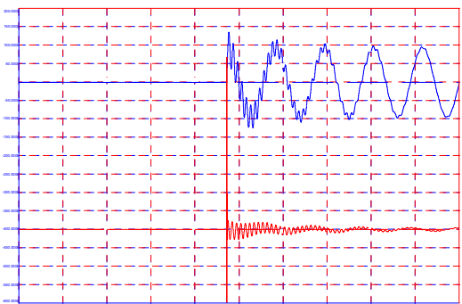
Voltage and Current for Energization of 2 nd Bank
