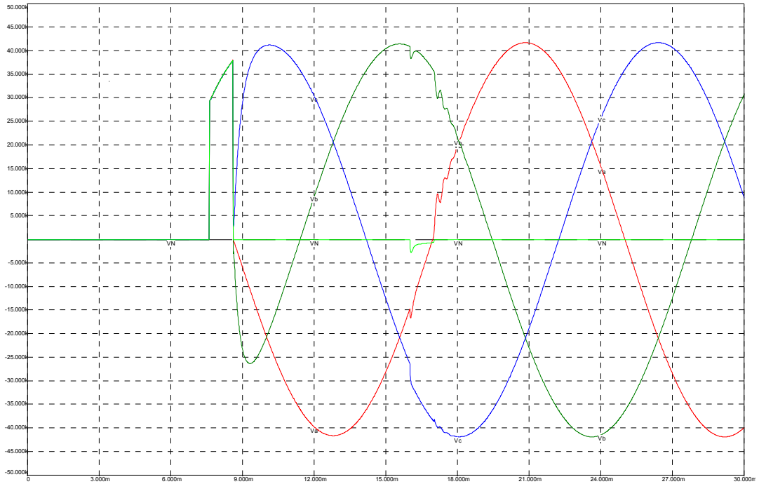
Capacitor Voltages from Simulation for U. S. Utility Installation of Capacitor Switch using Pre-Insertion Resistor
