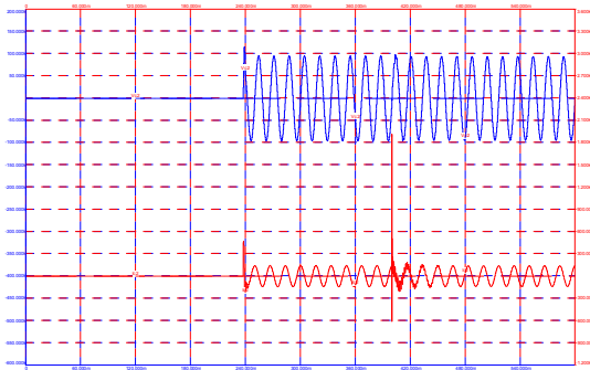
Voltage and Current for Energization of 2 nd Bank at 81 Ohms
