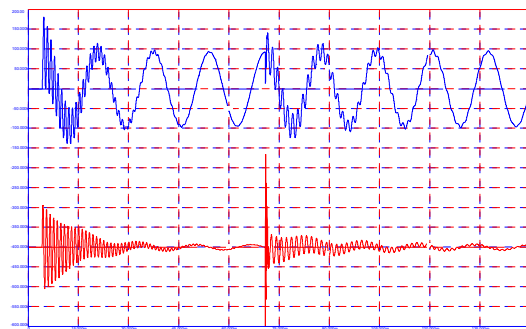
Voltages and Current for Energization of 1 st Bank
