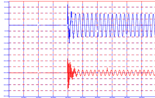
Voltage and Current for Energization of 2 nd Bank at 5.5 Ohms
