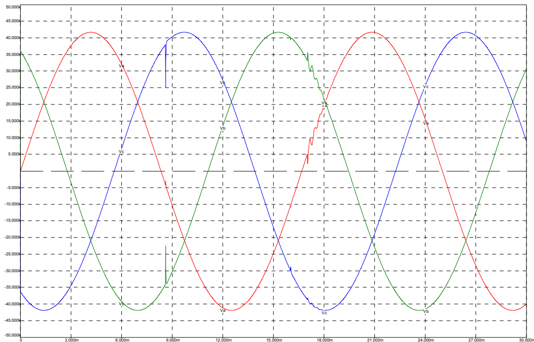
Substation Bus Voltages from Simulation for U. S. Utility Installation of Capacitor Switch using Pre-Insertion Resistor
