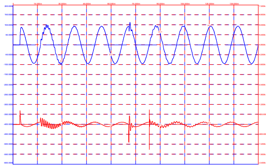
Voltage and Current for Energization of 1 st Bank at 80 Ohms
