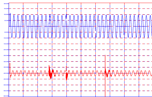
Voltage and Current for Energization of 1 st Bank at 81 Ohms
