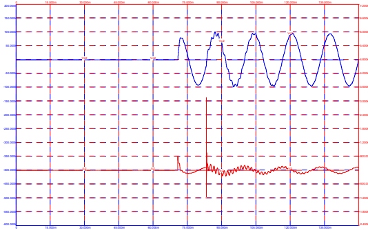
Voltage and Current for Energization of 2 nd Bank at 150 Ohms
