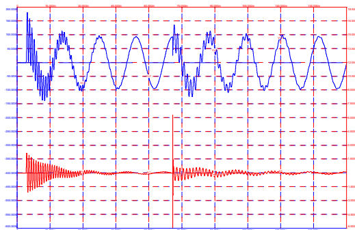
Voltage and Current for Energization of First Bank
