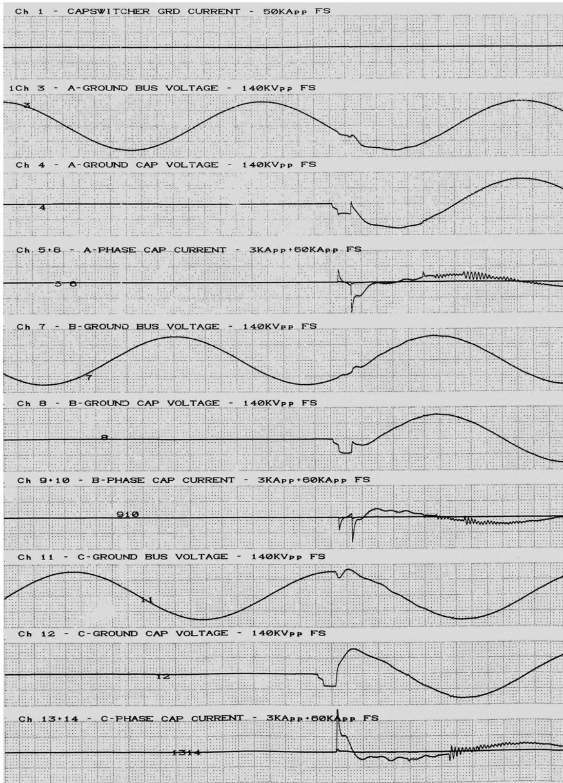
Oscillograph from Installation at U. S. Utility For CapSwitcher ® Capacitor Switch with Pre-Insertion Resistors
