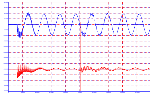
Voltage and Current for Energization of 1 st Bank
