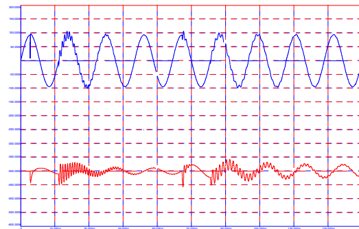
Voltage and Current for Energization of 1 st Bank at 150 Ohms
