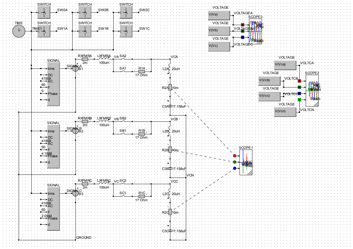
Simulation Model for Ungrounded Wye Capacitor Bank 72.5kV, 27.5MVAR installed at U. S. Utility
